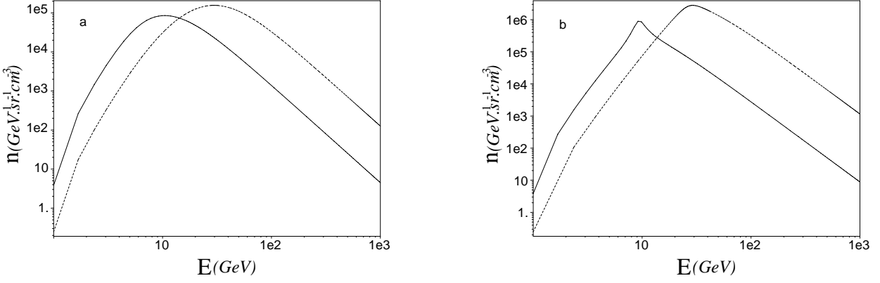
Fig. 1. Spectrum of protons in jets with \alpha = 2.5 , \Gamma = 10 (solid lines) and \Gamma = 30 (dash lines). In a ) \theta = 6^\circ and in b ) \theta = 0.6^\circ
