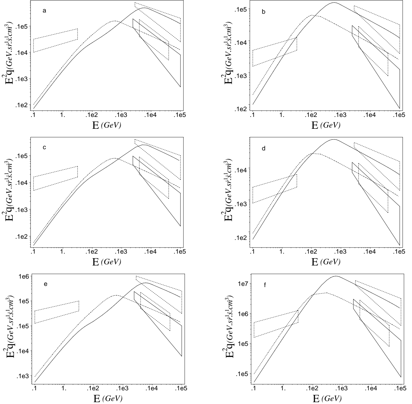
Fig. 4. The second model results: Predicted spectra for \theta = 6^\circ , \Gamma = 10 , E_2 = 100 GeV (dashed line), E_2 = 1000 GeV (solid line) and R = 6.5 \cdot 10^{13} cm in a ), E_2 = 100 GeV (solid line), E_2 = 20 GeV (dashed line) and R = 1.2 \cdot 10^{14} cm in b ), \Gamma = 30 , E_2 = 100 GeV (dashed line), E_2 = 1000 GeV (solid line) and R = 7.5 \cdot 10^{13} cm in c ), E_2 = 100 GeV (solid line), E_2 = 20 GeV (dashed line) and R = 1.5 \cdot 10^{14} cm in d ), \Gamma = 10 , \theta = 0.6^\circ , E_2 = 100 GeV (dashed line), E_2 = 1000 GeV (solid line) and R = 2.7 \cdot 10^{13} cm in e ), \Gamma = 30 , \theta = 0.6^\circ , E_2 = 100 GeV (solid line), E_2 = 20 GeV (dashed line) and R = 1.2 \cdot 10^{13} cm in f ) are compared to data of Mrk 421 as in Fig. 3. See Sect. 3 for details
