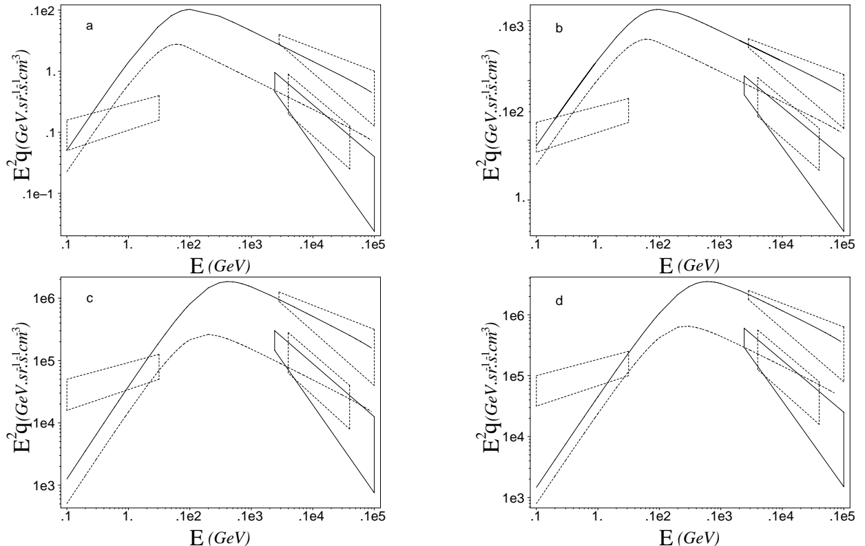
Fig. 3. The first model results: The spectra for \theta = 6^\circ and different \Gamma 's are compared to data of Mrk 421 in GeV range (Lin et al. 1994) and TeV low state (Mohanty et al. 1993; dashed box and Piron 2000; solid box) and high state (McEney et al. 1997), as error boxes. \Gamma_1 = 2 (dashed line), \Gamma_2 = 100 (solid line) and R = 1.7 \cdot 10^{15} cm in a ), \Gamma_1 = 4 (dashed line), \Gamma_2 = 30 (solid line) and R = 6.7 \cdot 10^{14} cm in b ), \theta = 0.6^\circ , \Gamma_1 = 30 (dashed line), \Gamma_2 = 60 (solid line) and R = 2.5 \cdot 10^{13} cm in c ), \Gamma_1 = 40 (dashed line), \Gamma_2 = 90 (solid line) and R = 2 \cdot 10^{13} cm in d ). See Sect. 2 for details
