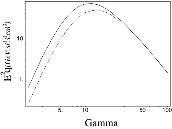
Fig. 2. Dependence of \gamma -ray emissivity on bulk Lorentz factor for E_\gamma = 1 GeV (solid line) and E_\gamma = 1 TeV (dashed line) and \theta = 6^\circ . From this plot one can find some values of \Gamma_1 and \Gamma_2 which give nearly identical emissivities at 1 GeV but different emissivities at 1 TeV
